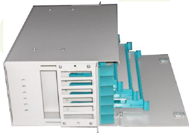
Optical Distribution Frame with Trays
